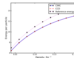
Figure: CCD, Reference energy and Diffusion Monte Carlo results for pure neutron matter with 66 neutrons and N_{\text{max}} = 36 .
